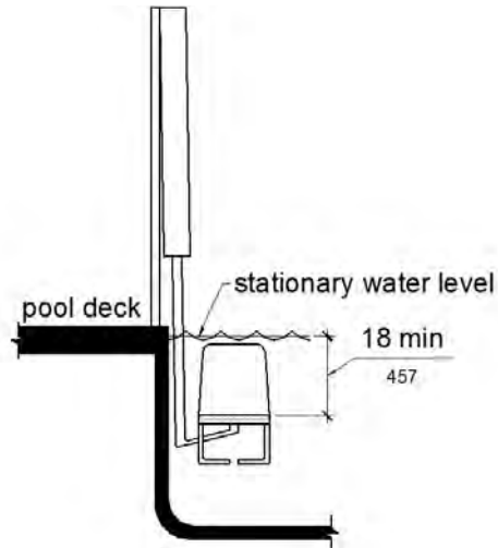
Figure 11B-1009.2.8 Pool Lift Submerged Depth
