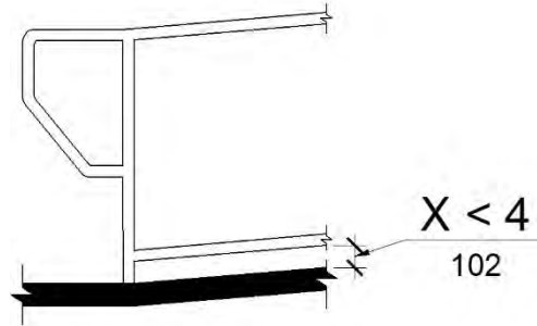
Figure 11B-405.9.2 Curb or Barrier Edge Protection
