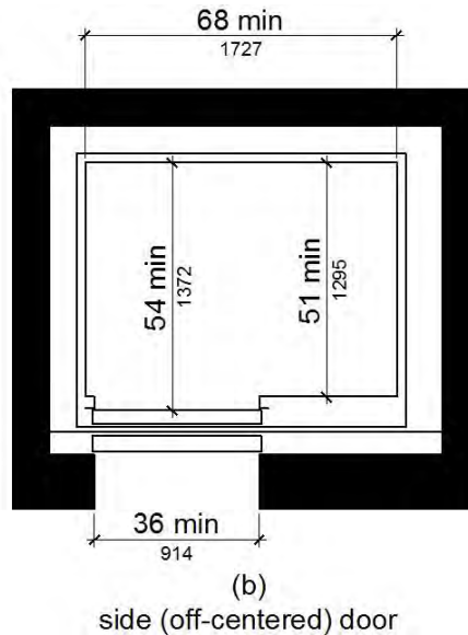
Figure 11B-407.4.1 Elevator Car Dimensions
