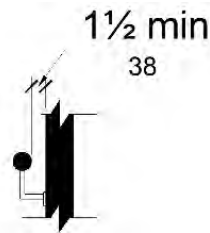
Figure 11B-505.5 Handrail Clearance
