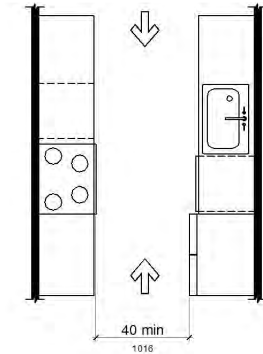
Figure 11B-804.2.1 Pass Through Kitchens
